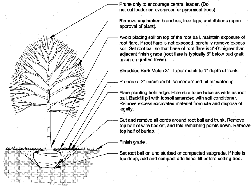
1 Deciduous Tree Planting d-tree-dec 1/2" = 1'-0"
