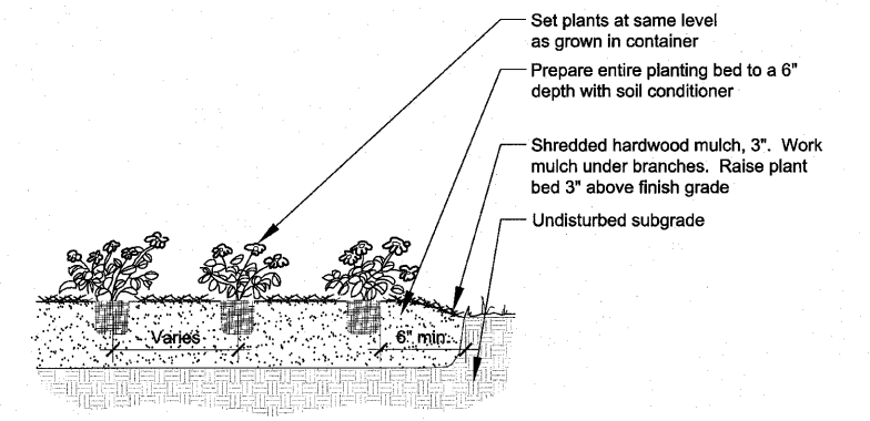
4 Perennial Planting d-annual-perennial 1/2" = 1'-0"
