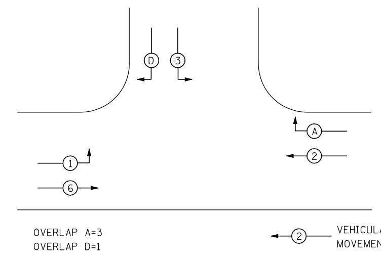
PHASE DESIGNATION DIAGRAM REFER TO STANDARD 857001
