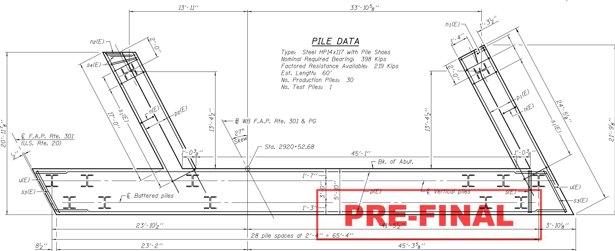
PLAN-PILE CAP
