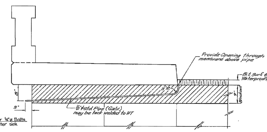
DRAIN HOLES AT EXPANSION JOINT
