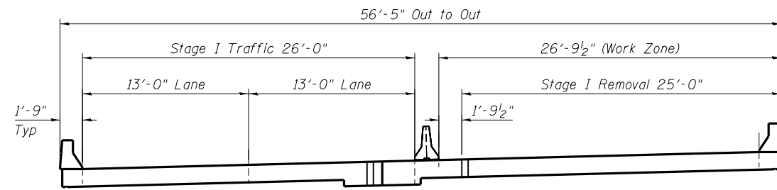
SN 082-0165 WESTBOUND CROSS SECTION (Looking East) STAGE I REMOVAL
