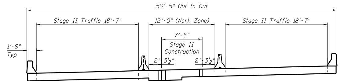
SN 082-0165 WESTBOUND CROSS SECTION (Looking East) STAGE II CONSTRUCTION
