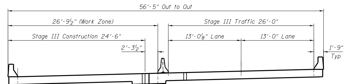
SN 082-0165 WESTBOUND CROSS SECTION (Looking East) STAGE III CONSTRUCTION
