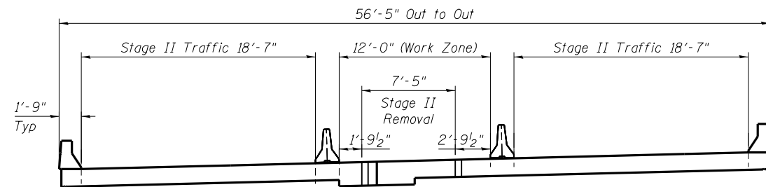
SN 082-0165 WESTBOUND CROSS SECTION (Looking East) STAGE II REMOVAL
