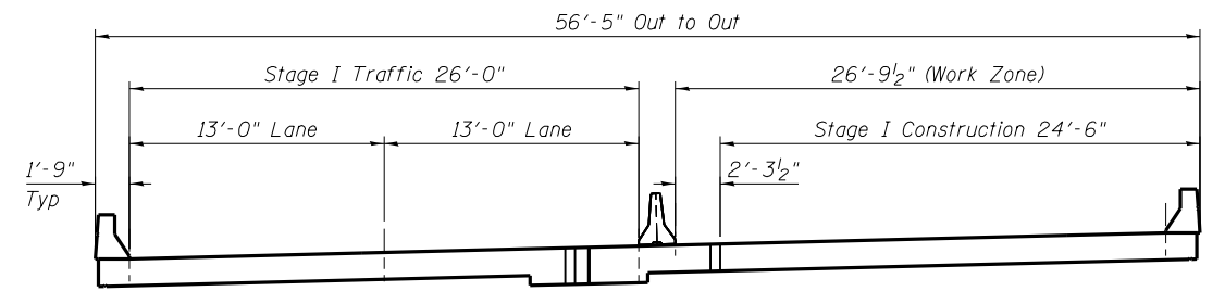
SN 082-0165 WESTBOUND CROSS SECTION (Looking East) STAGE I CONSTRUCTION
