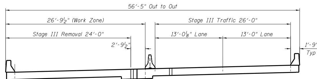
SN 082-0165 WESTBOUND CROSS SECTION (Looking East) STAGE III REMOVAL
