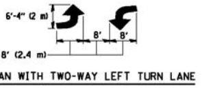
MEDIAN WITH TWO-WAY LEFT TURN LANE
