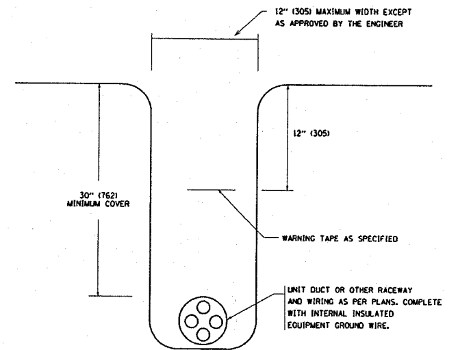
TYPICAL WIRING IN TRENCH DETAIL
