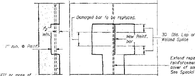
CONCRETE REPAIR DETAIL
