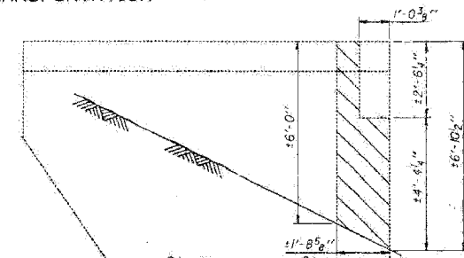
N. Abut. W. Wing - East Structure
