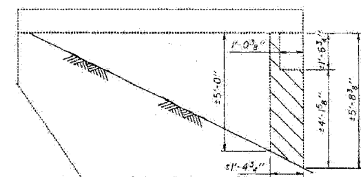
S. Abut. E. Wing - East Structure
