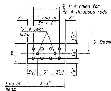
TOP PLATE
