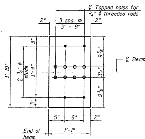
BOTTOM PLATE
