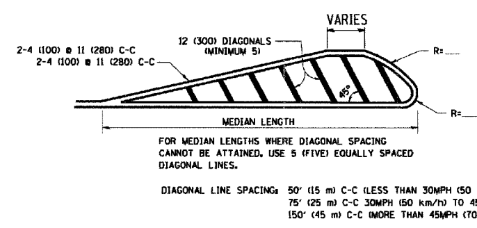
MEDIANS OVER 4' (1.2 m) WIDE
