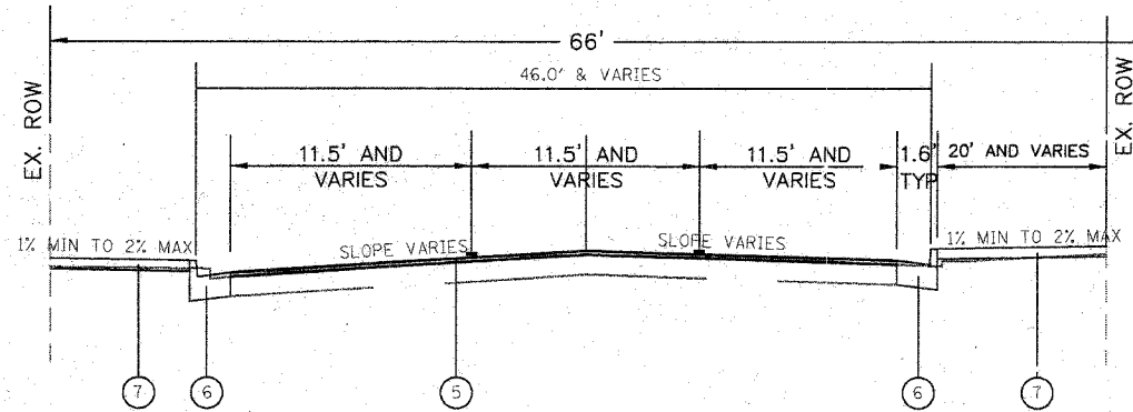
MAIN STREET (EAST & WEST) PROPOSED TYPICAL SECTION STA. 25+76.41 TO STA. 28+26.85 STA. 31+14.46 TO STA. 33+55.08
