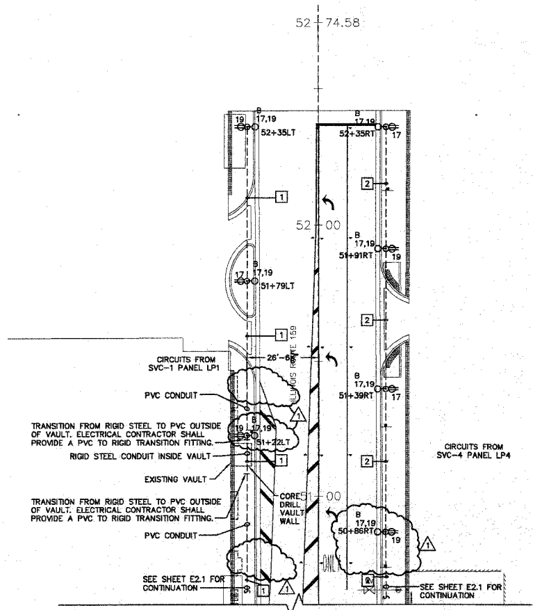
NORTH ELECTRICAL PLAN - LIGHTING 1" = 20'-0"
