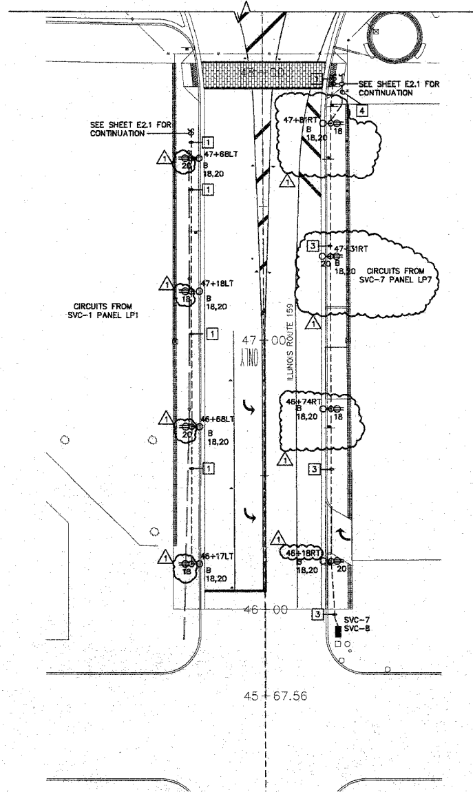
SOUTH ELECTRICAL PLAN - LIGHTING 1" = 20'-0"
