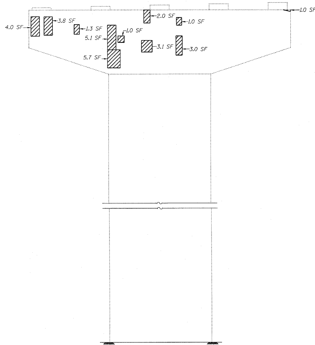
ELEVATION (Looking South)
