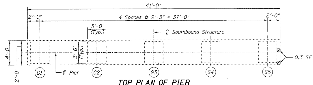
TOP PLAN OF PIER
