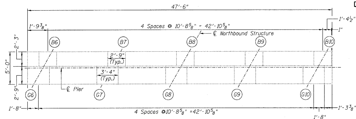
TOP PLAN OF PIER
