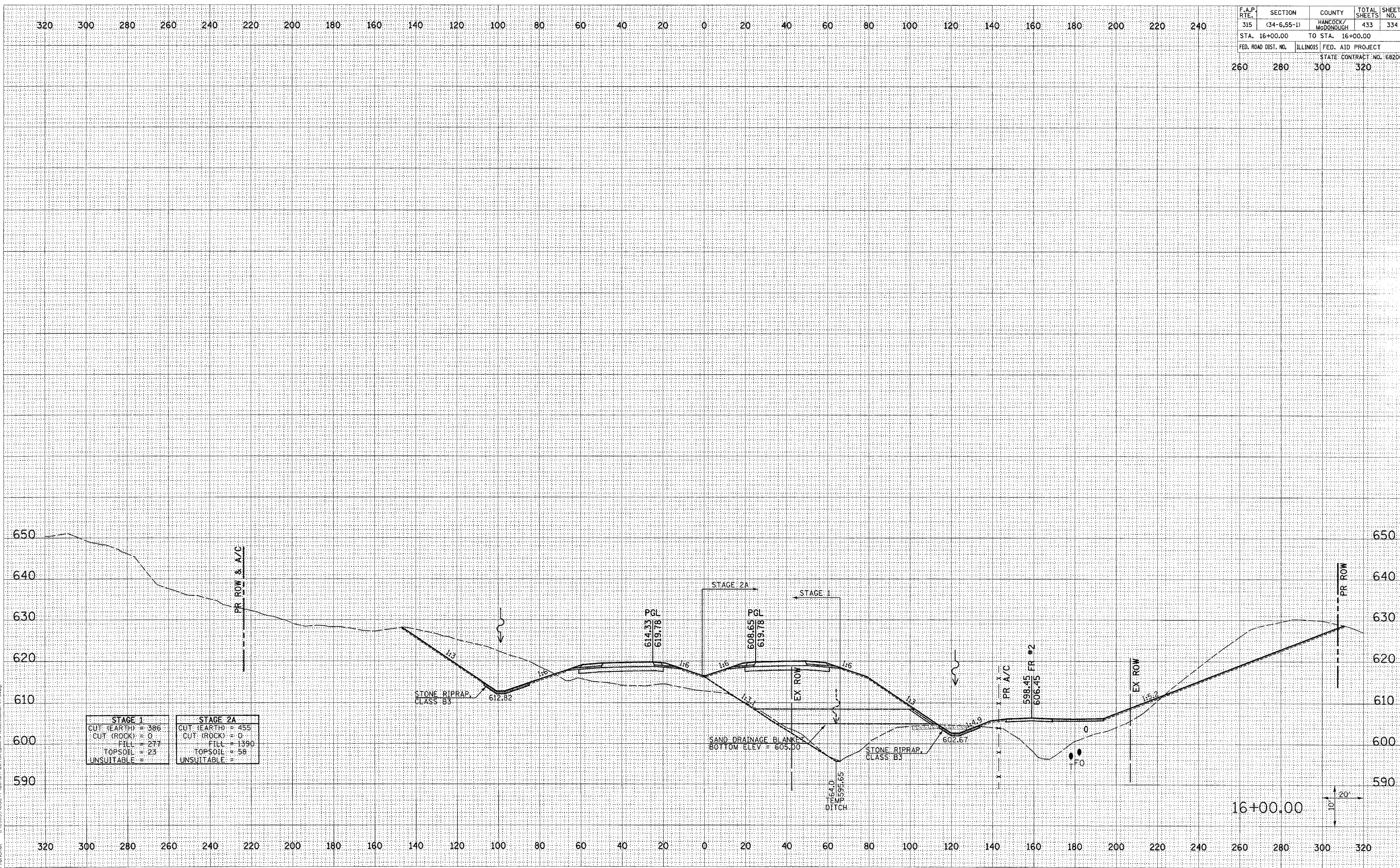
FAP ROUTE 315 (IL 336) CROSS SECTIONS STA 16+00.00 TO 16+00.00
