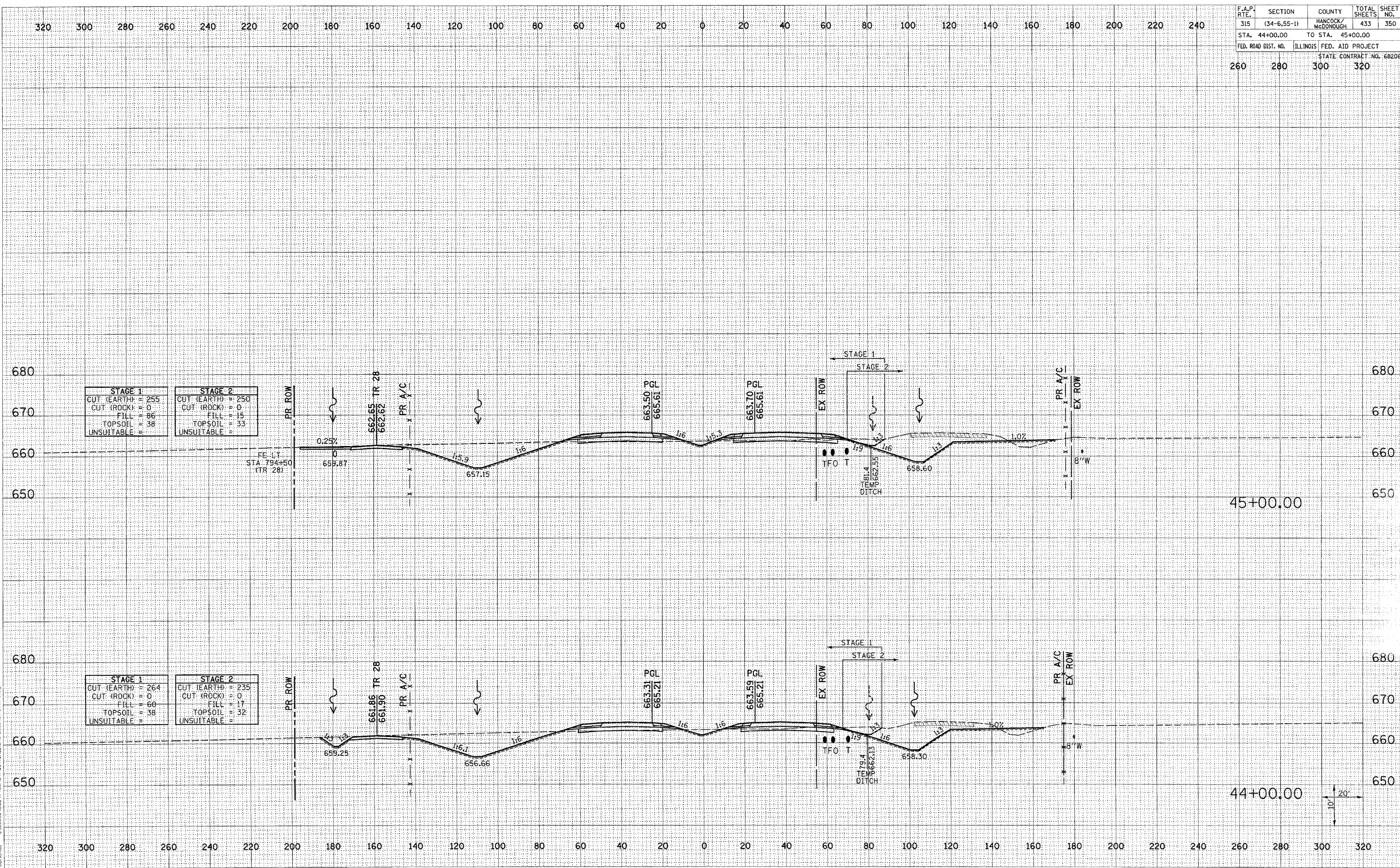
FAP ROUTE 315 (IL 336) CROSS SECTIONS STA 44+00.00 TO 45+00.00
