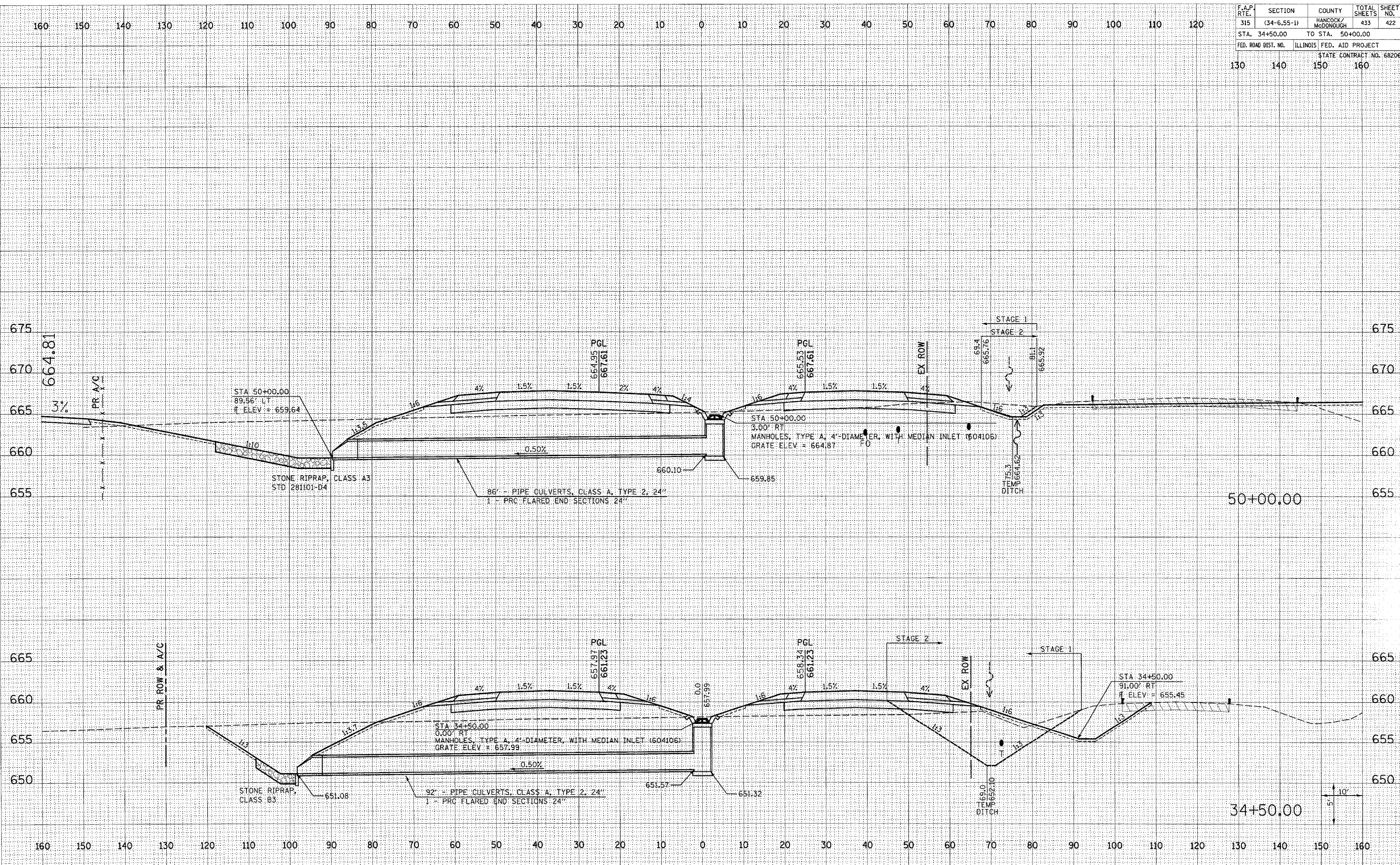
FAP 315 (IL 336) DRAINAGE CROSS SECTIONS STA 34+50.00 TO 50+00.00
