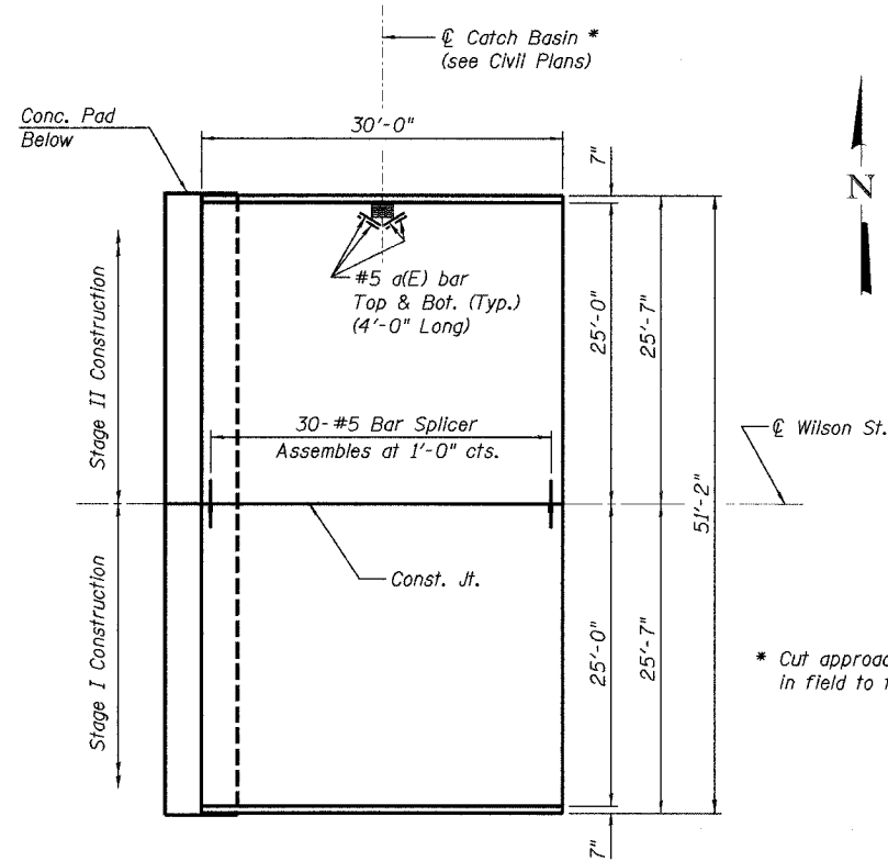
PLAN - WEST APPROACH SLAB
