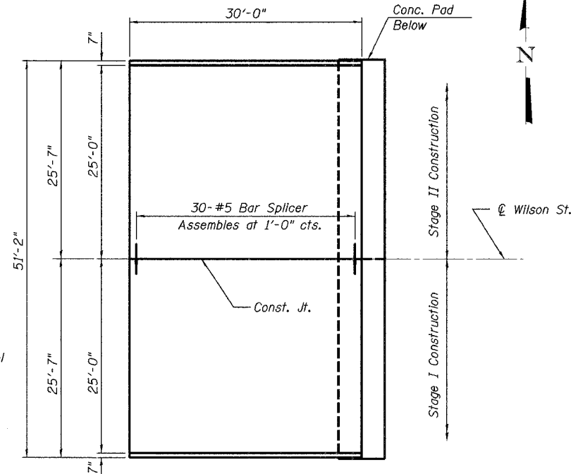
PLAN - EAST APPROACH SLAB
