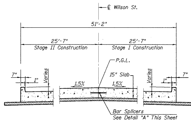
TYPICAL SECTION THRU APPROACH PAVEMENT (Looking East)
