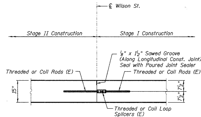
DETAIL "A" (Looking East)
