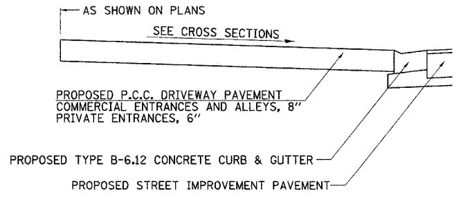
CROSS SECTION
