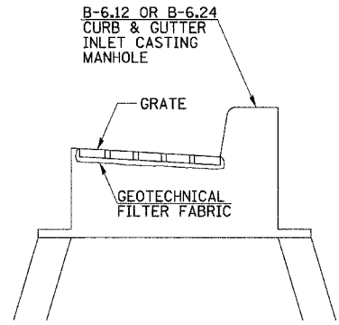
FILTER FABRIC-INLET PROTECTION DETAIL TO BE PAID FOR AT THE CONTRACT UNIT PRICE "EACH" FOR "FILTER FABRIC-INLET PROTECTION"
