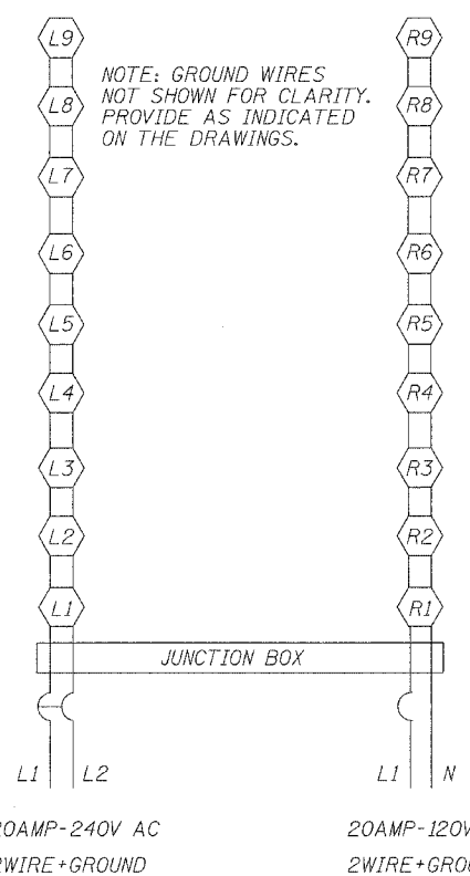
LIGHTING AND RECEPTACLE WIRING SCHEMATIC - SOUTH SIDE OF BRIDGE
