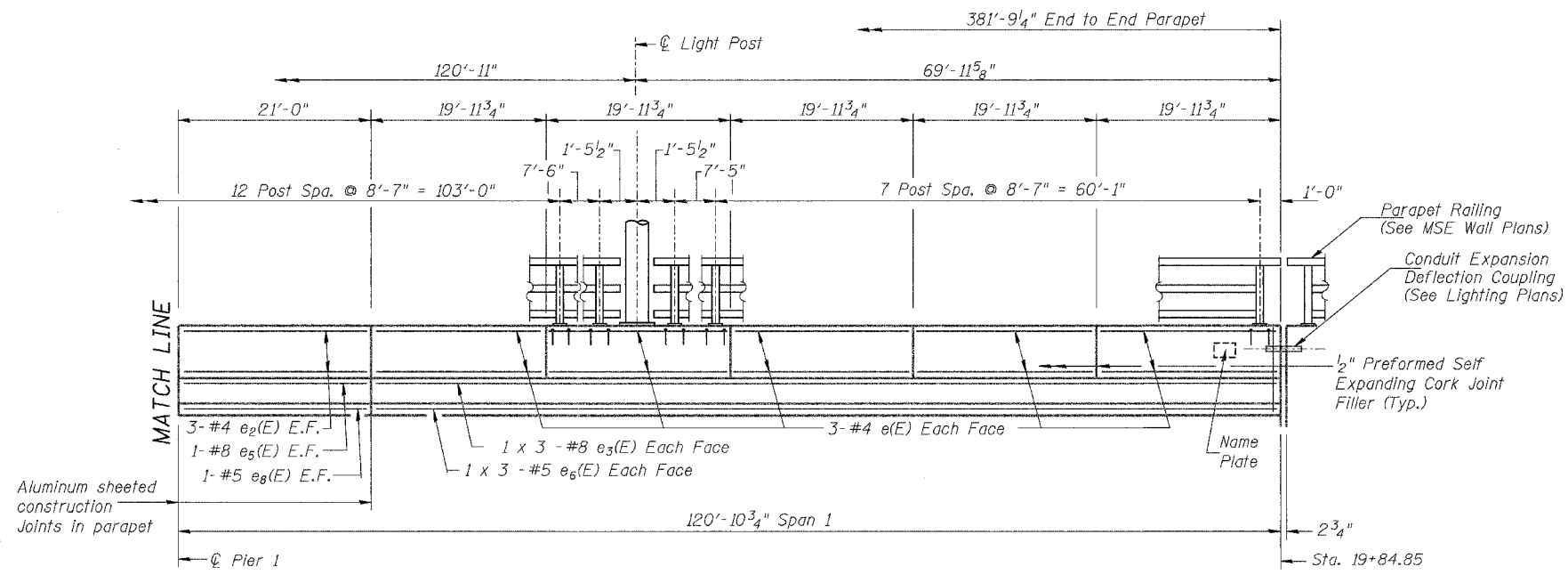
PARAPET ELEVATION (SOUTH TRAFFIC BARRIER) (Looking South at South Roadway Parapet)
