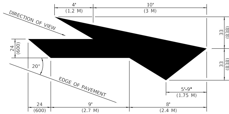
LANE-REDUCTION ARROW
