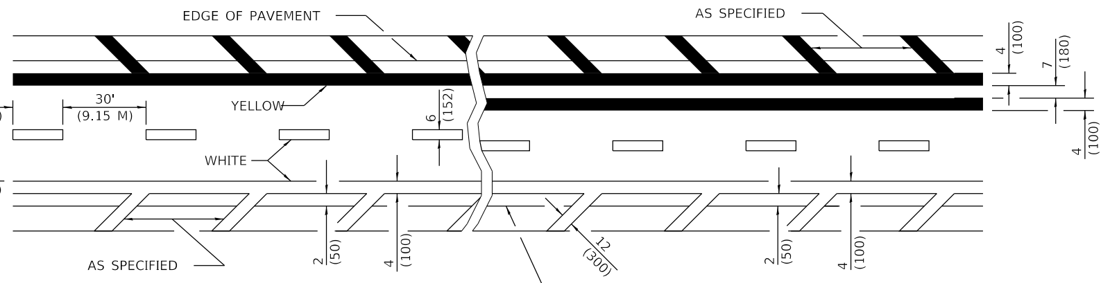
MULTI LANE
