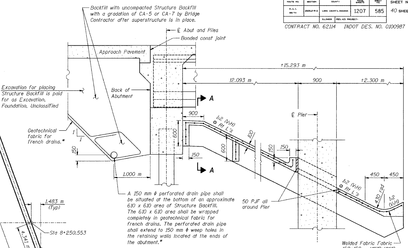
SECTION THRU ABUTMENT (Dimensions at Right Angles)
