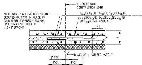
CROSS SECTION THRU LONGITUDINAL CONSTRUCTION JOINT BETWEEN LANE LINES
