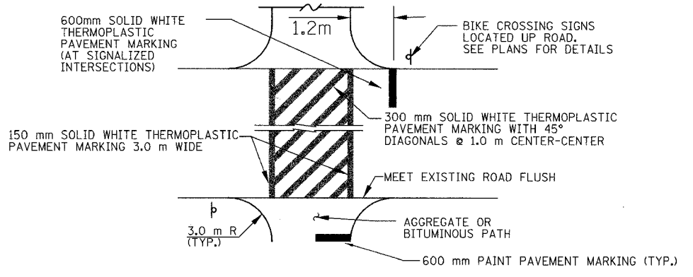
PAVEMENT MARKING DETAIL
