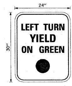
MAST ARM MOUNTED SIGN DETAILS NO SCALE MUTCD R10-12
