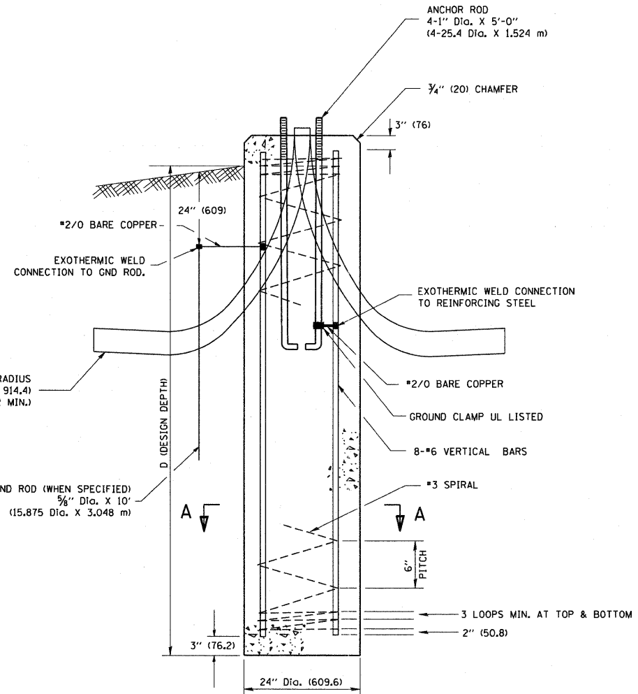
FOUNDATION DETAIL
