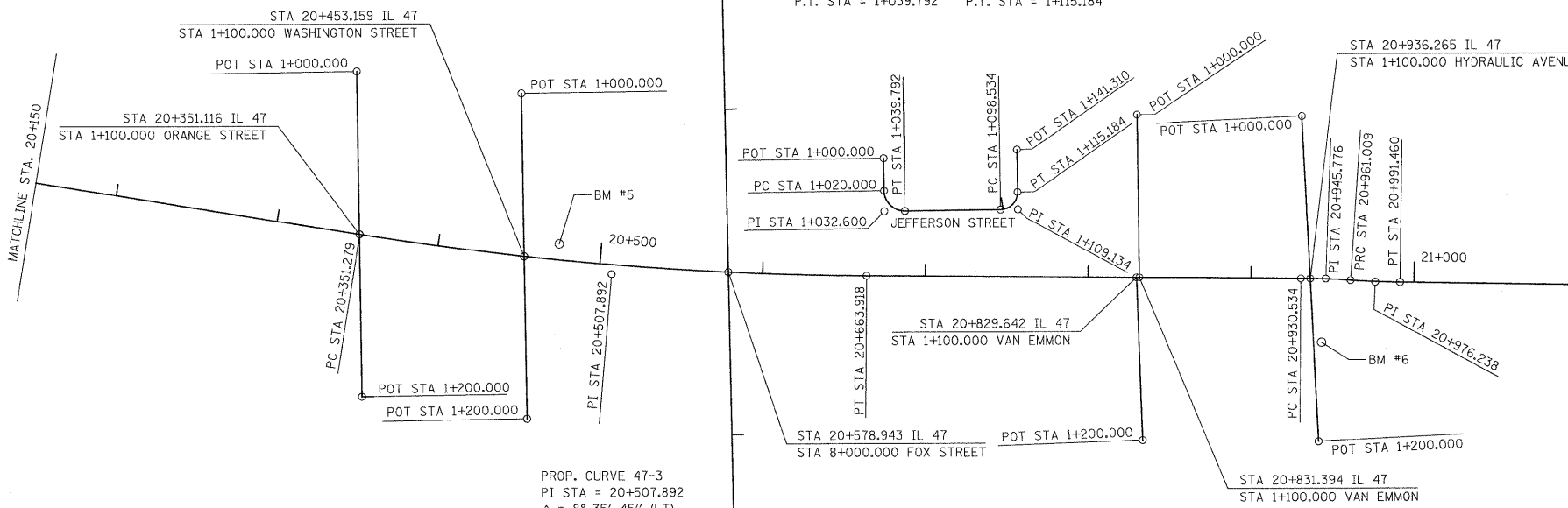
CENTERLINE VAN EMMON STREET (WEST)
