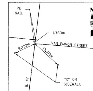
CENTERLINE VAN EMMON STREET (EAST)
