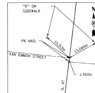
CENTERLINE VAN EMMON STREET (WEST)
