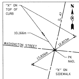
CENTERLINE WASHINGTON STREET
