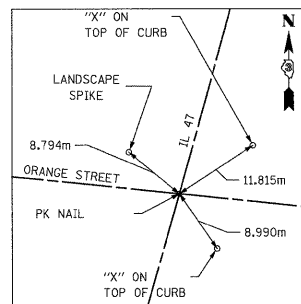
CENTERLINE ORANGE STREET
