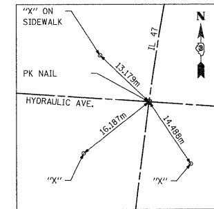
CENTERLINE HYDRAULIC AVENUE
