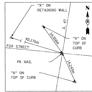
CENTERLINE FOX STREET
