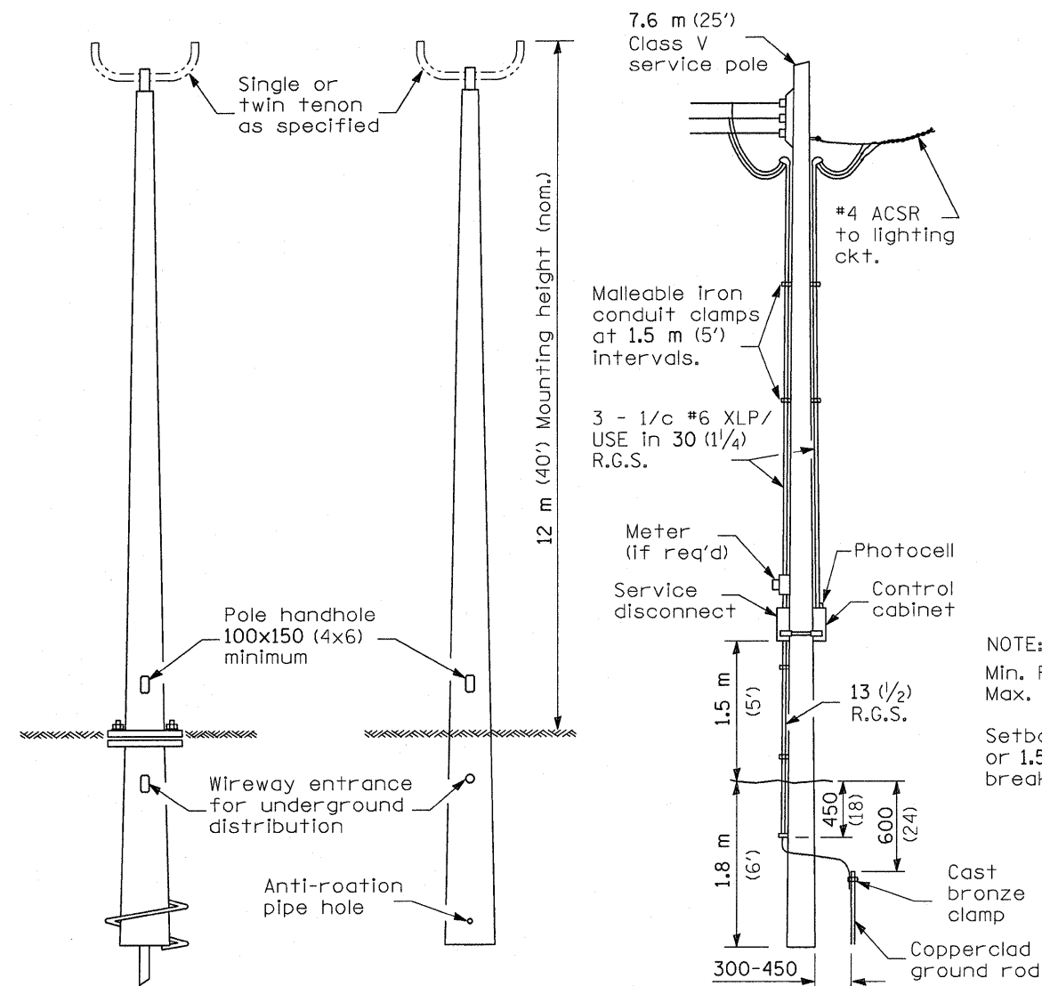
ANCHOR BASE W/ METAL FOUNDATION BUTT BASE POLE, FIBERGLASS BREAKAWAY TYPE
