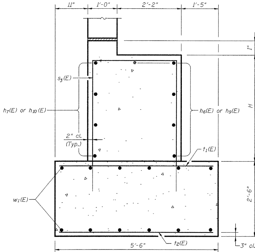
SECTION C-C
