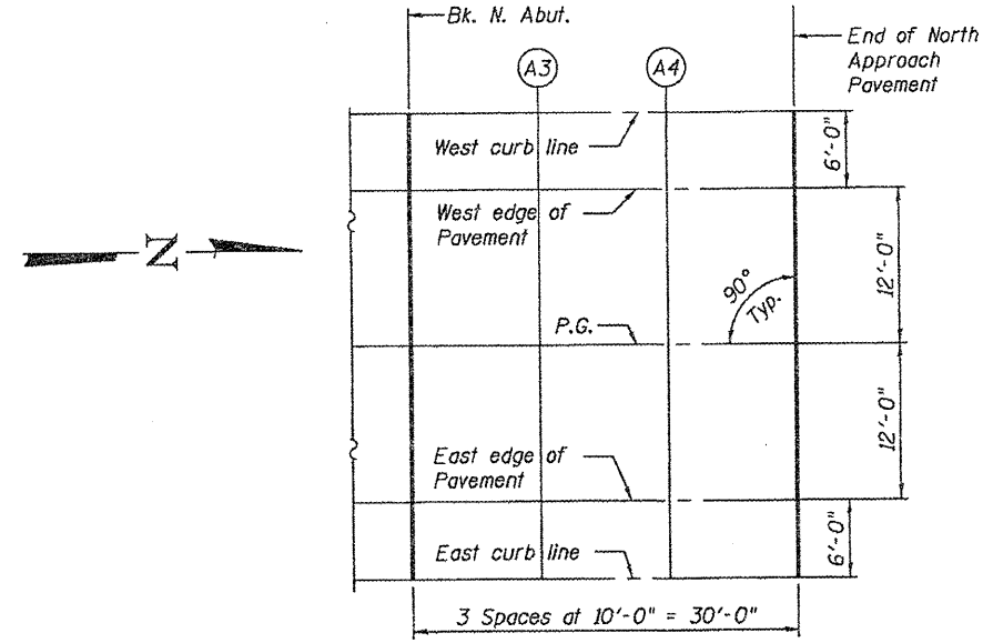
NORTH APPROACH PAVEMENT PLAN
