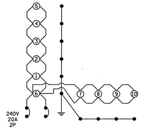
CIRCUIT DIAGRAM - EAST CROSSOVER
