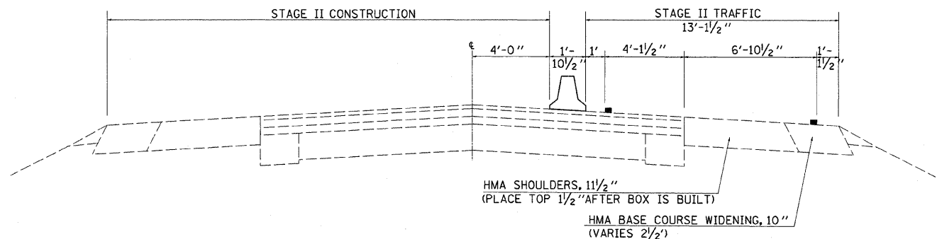
STAGE II - CULVERT NO. 2
