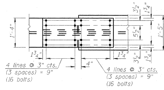
FIELD SPLICE 11 DETAIL (6 Required)
