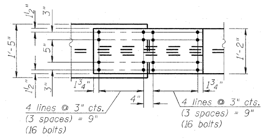
FIELD SPLICE 12A DETAIL (6 Required)
