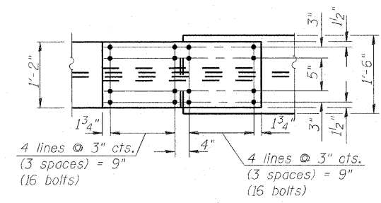
FIELD SPLICE 12B DETAIL (6 Required)
