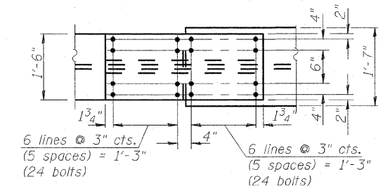
FIELD SPLICE 5B DETAIL (5 Required)
