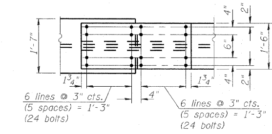
FIELD SPLICE 5A DETAIL (5 Required)
