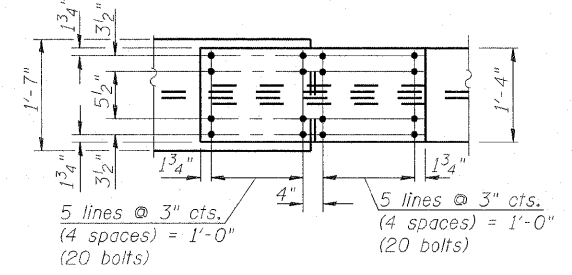
FIELD SPLICE 6 DETAIL (5 Required)
