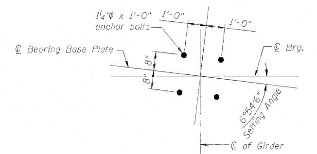
ANCHOR BOLT LOCATION DETAIL ABUTMENT BILL OF MATERIAL
