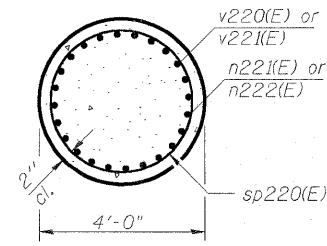
SEC. C-C
