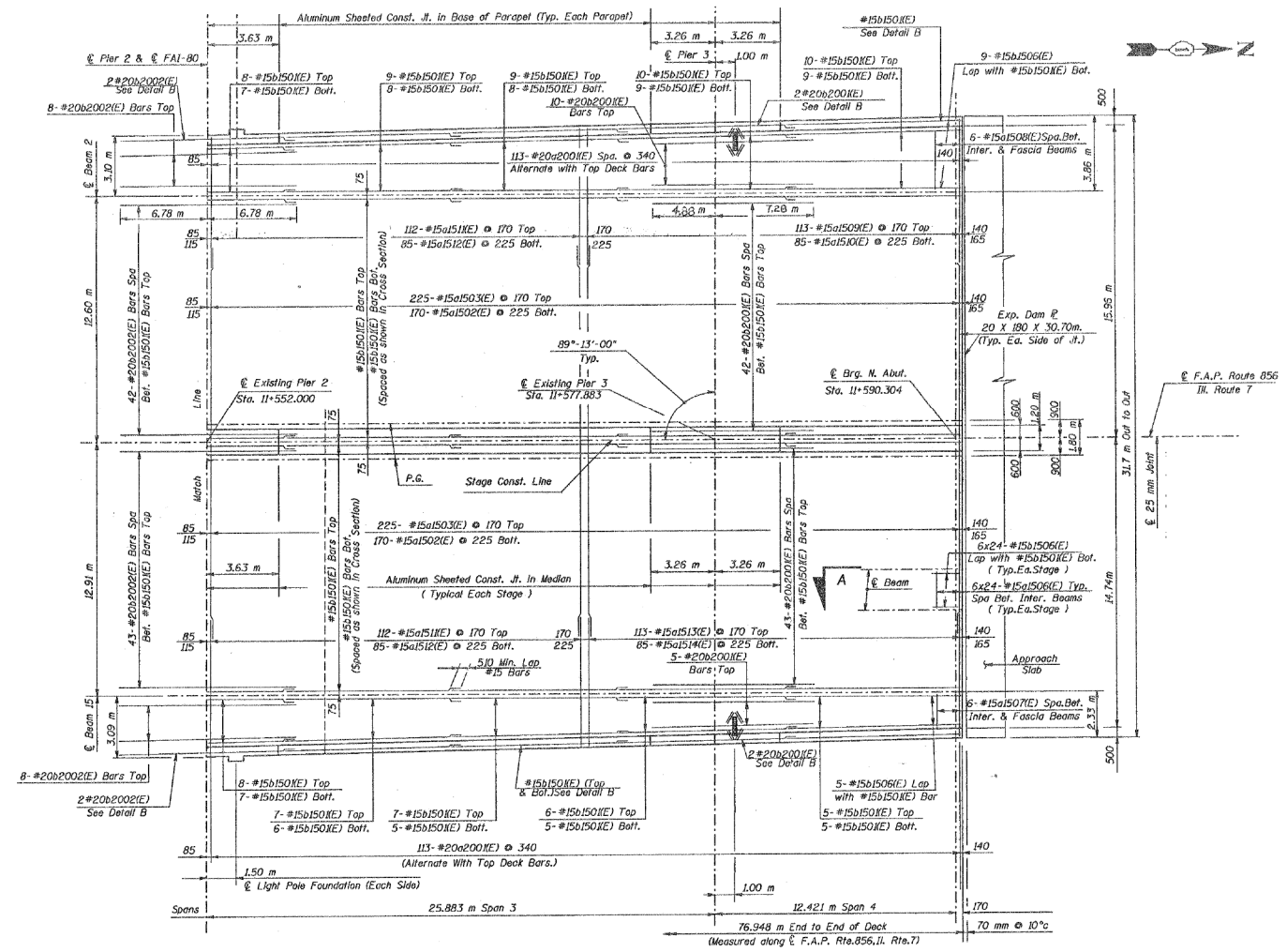
DECK PLAN
