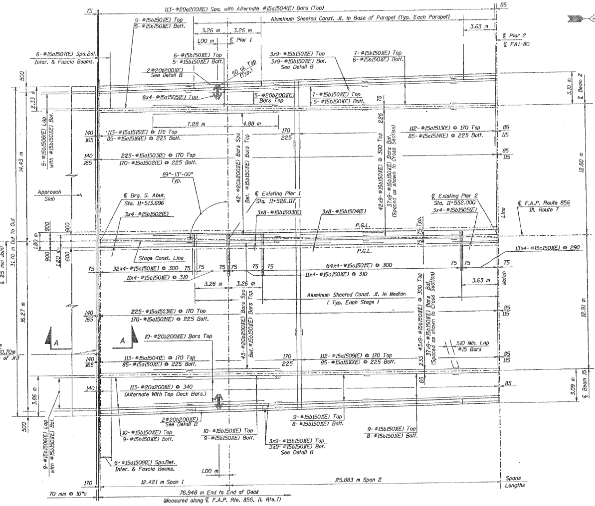
DECK PLAN
