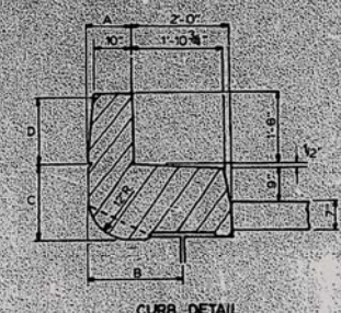
CURB DETAIL
