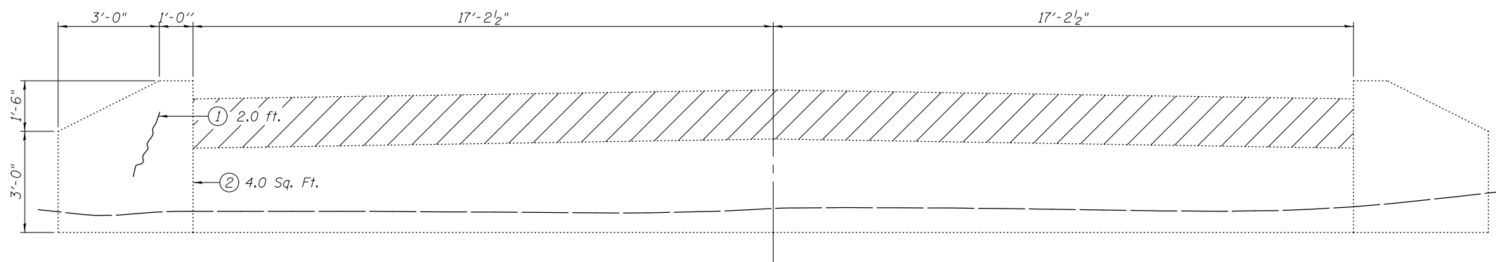
WEST ABUTMENT ELEVATION
