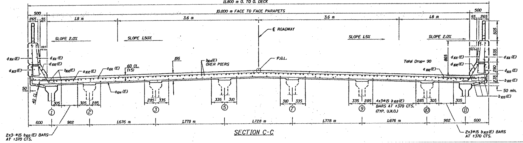
EXISTING TYPICAL SECTION SN 022-0089
