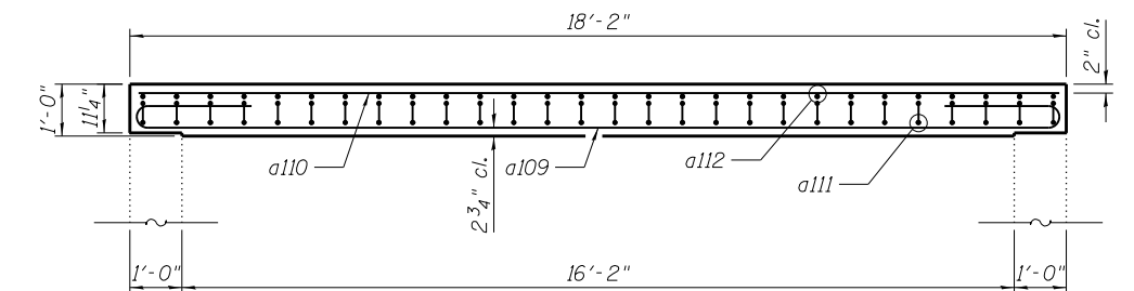
SECTION B-B
