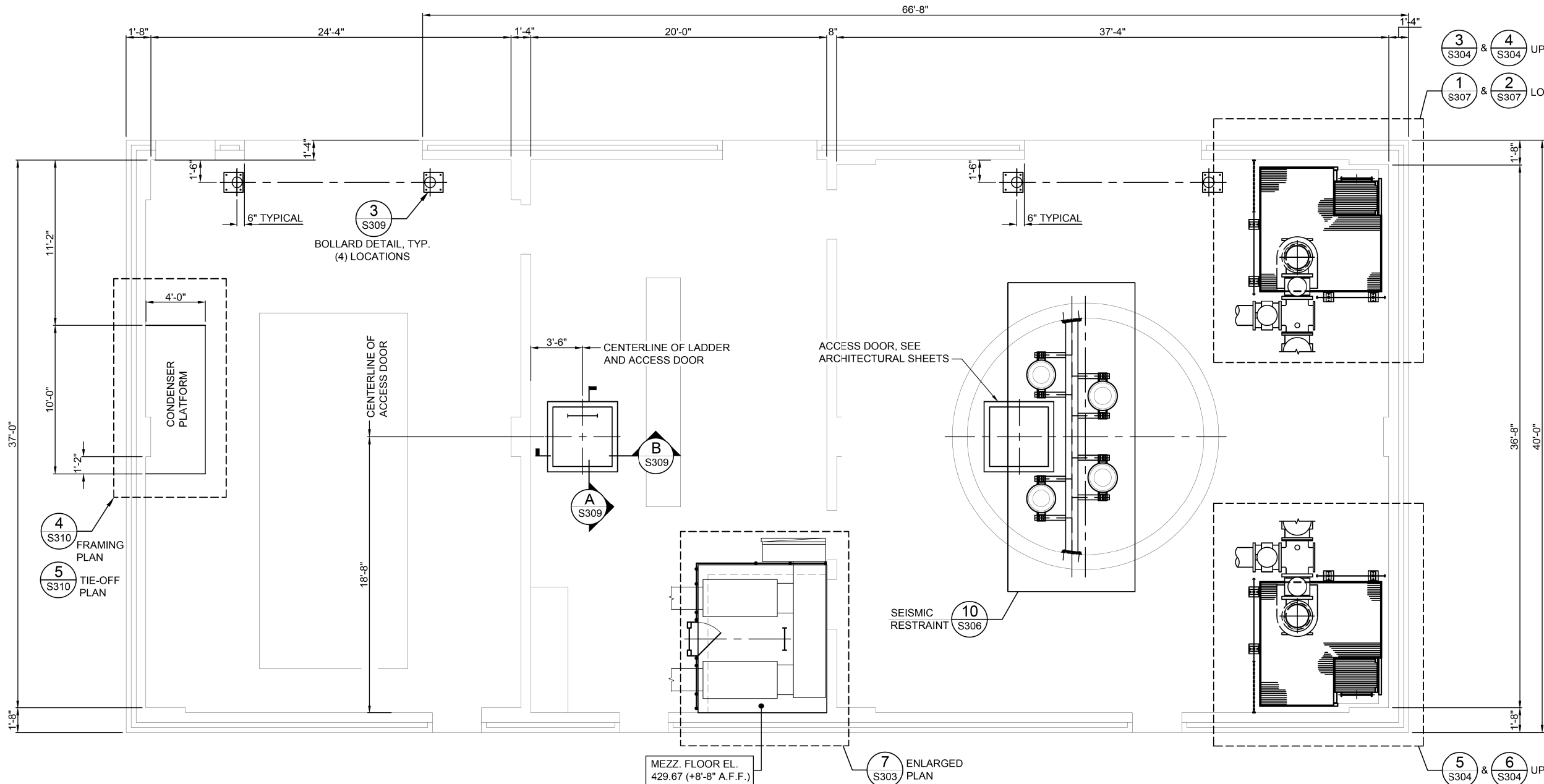
LOWER FRAMING PLAN SCALE: 1/4" = 1'-0"
