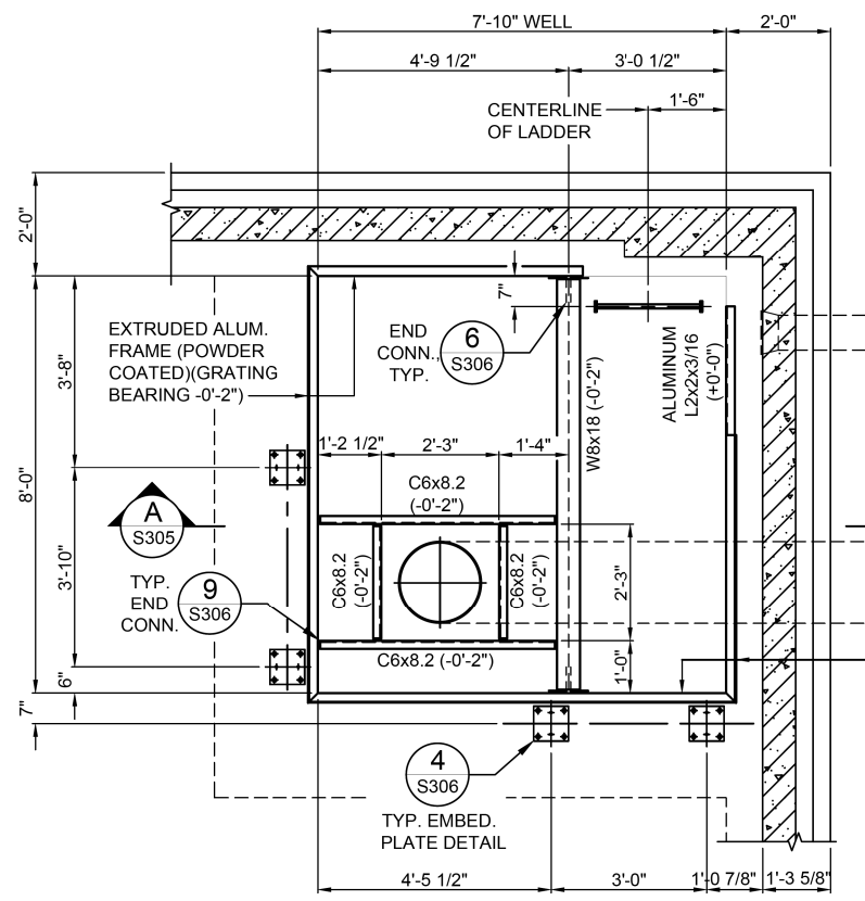
3 SOUTHEAST COLLECTOR WELL FRAMING PLAN S304 SCALE: 1/2"=1'-0" FIN. FLOOR EL. 421.00 (+0'-0")
