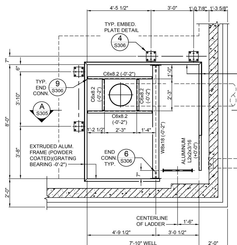
5 SOUTHWEST COLLECTOR WELL FRAMING PLAN S304 SCALE: 1/2"=1'-0" FIN. FLOOR EL. 421.00 (+0'-0")
