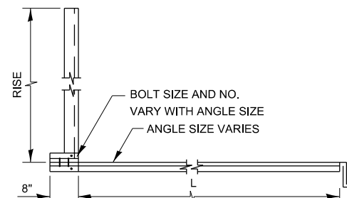
SECTION VIEW
