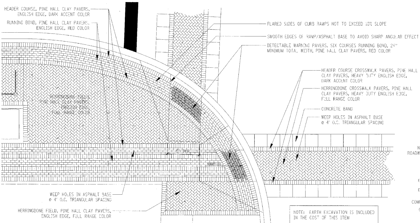
BRICK PAVERS / CURB RAMPS PLAN 1/4" = 1'-0"
