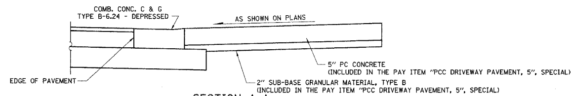
SECTION A-A PCC RESIDENTIAL DRIVEWAY DETAIL NOT TO SCALE
