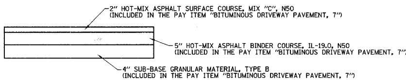
HOT-MIX ASPHALT COMMERCIAL DRIVEWAY DETAIL NOT TO SCALE
