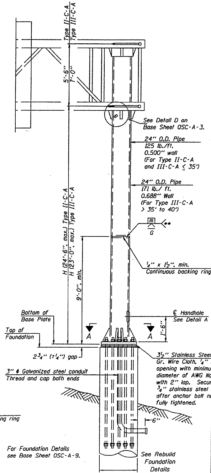
FRONT ELEVATION
