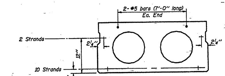
CROSS SECTION (35' SPAN)
